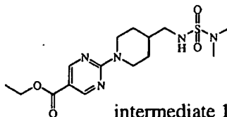
intermediate 11
